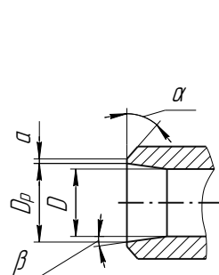
DN 20
