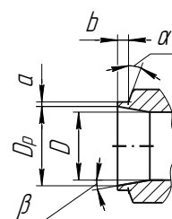
DN 32, 50
